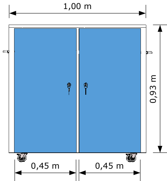
Vista frontal
